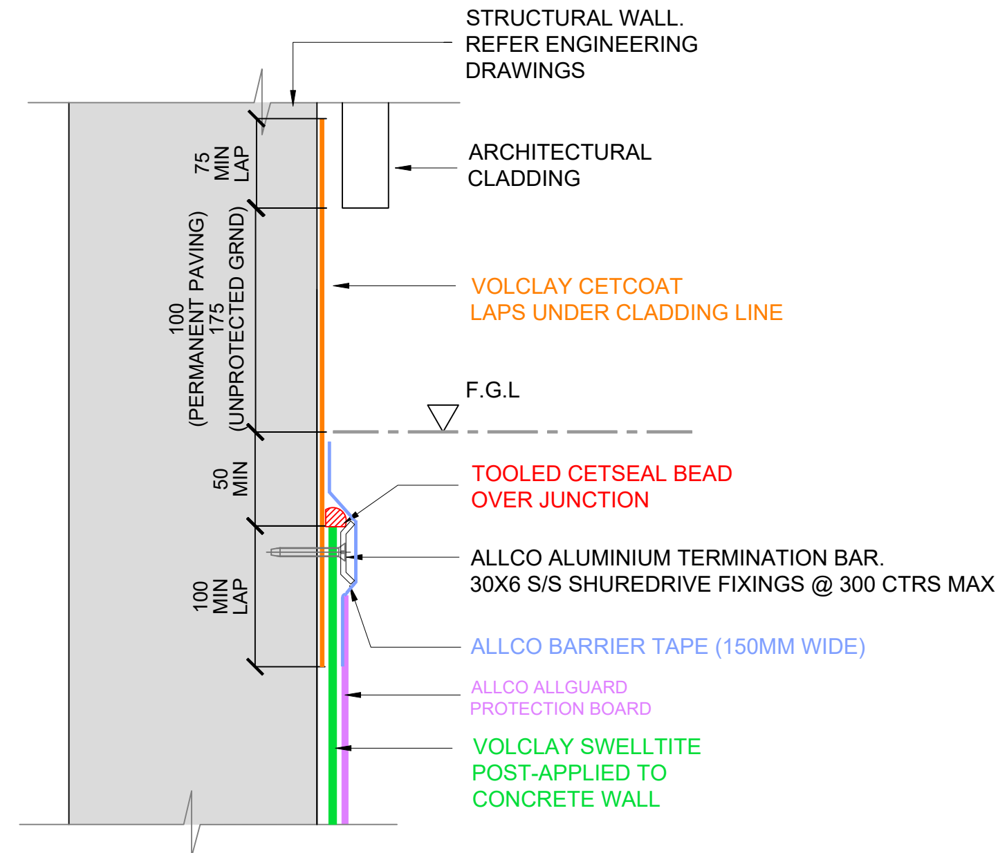
1 TERMINATION (F.G.L) - SWELLTITE - SPECIAL OPTION SCALE: NTS
