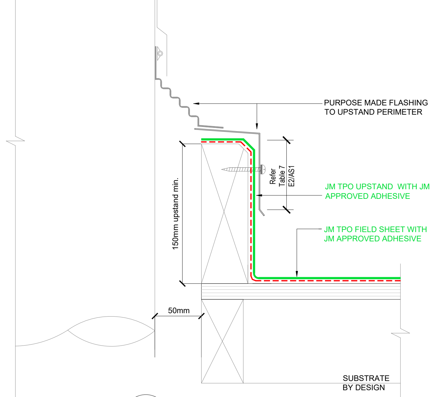
A FLUE / EXTRACT UPSTAND
