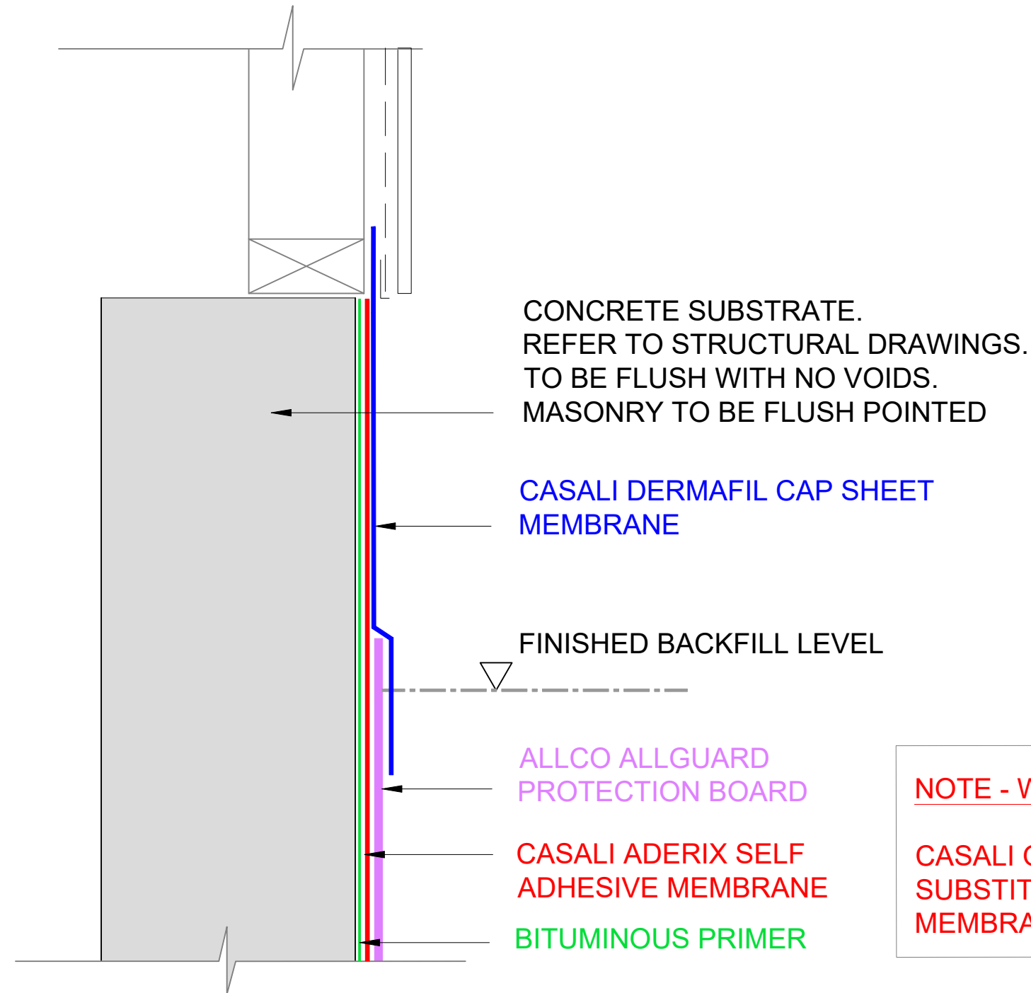
1 TERMINATION - BEHIND CLADDING SCALE: NTS
