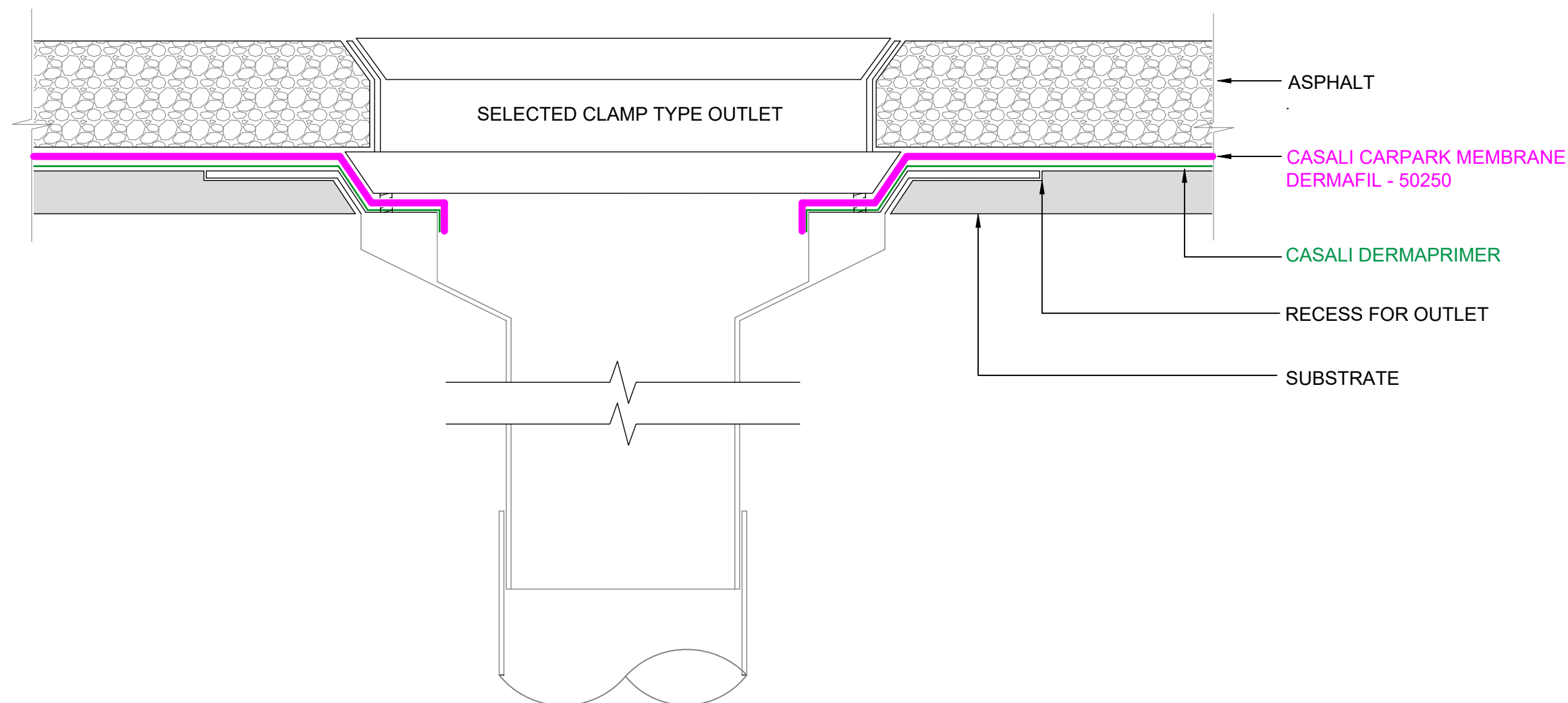
1 CARPARK MEMBRANE - EXPANSION DRAINAGE OUTLET SCALE: NTS
