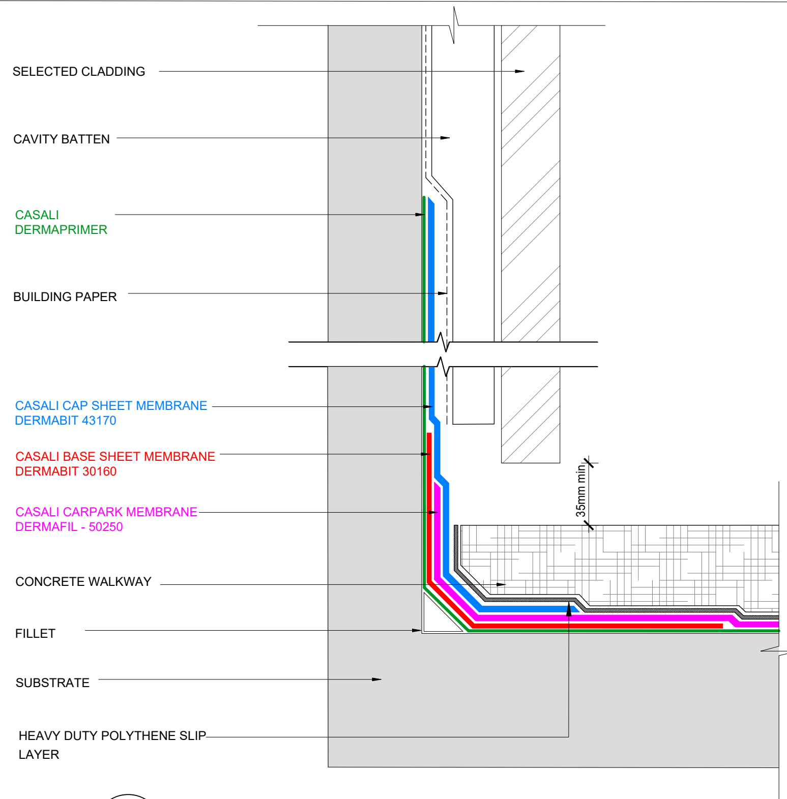
CARPARK MEMBRANE - UPSTAND BEHIND CAVITY
