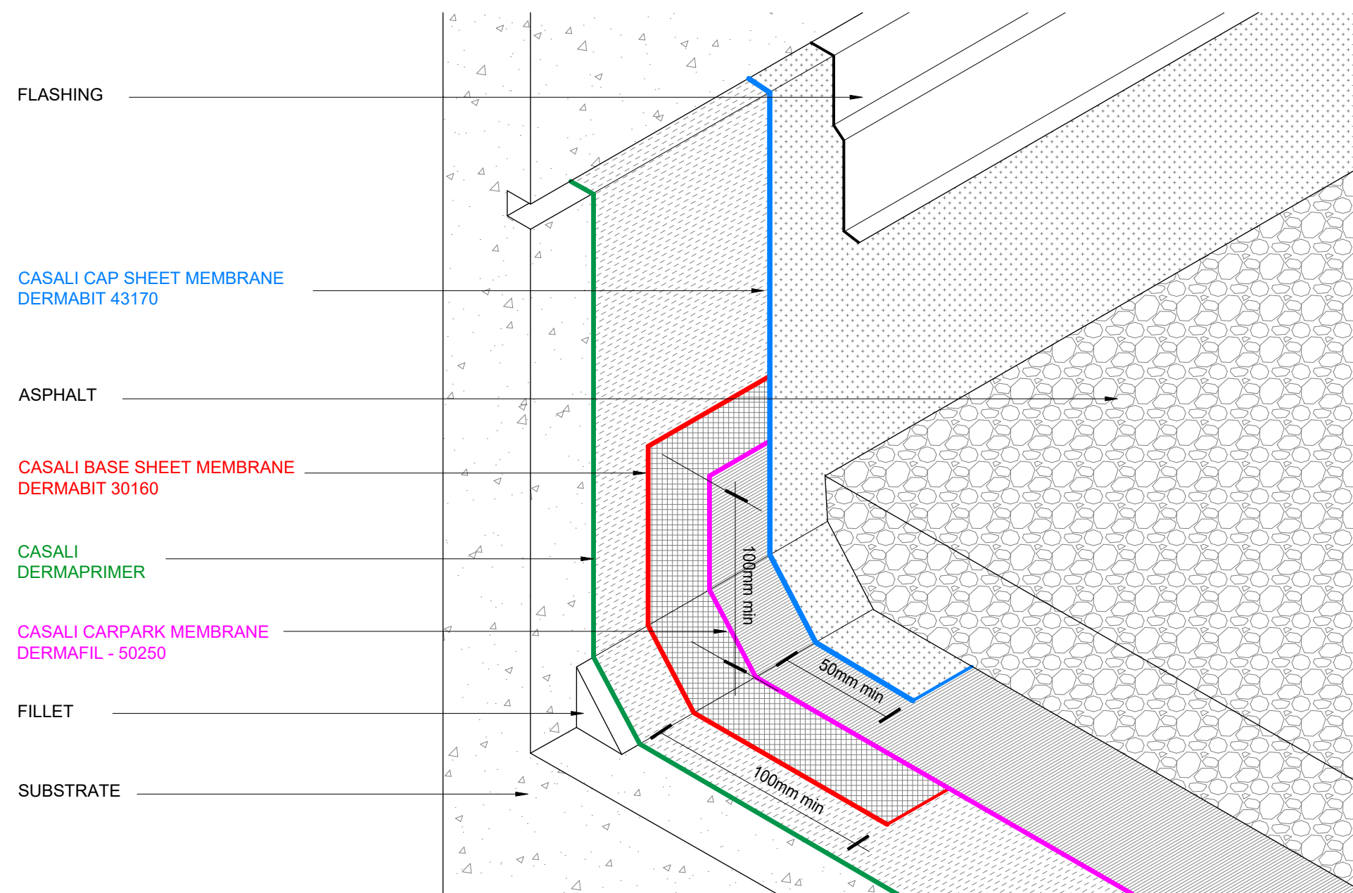
1 CARPARK MEMBRANE - TERMINATION INTO CHASE SCALE: NTS
