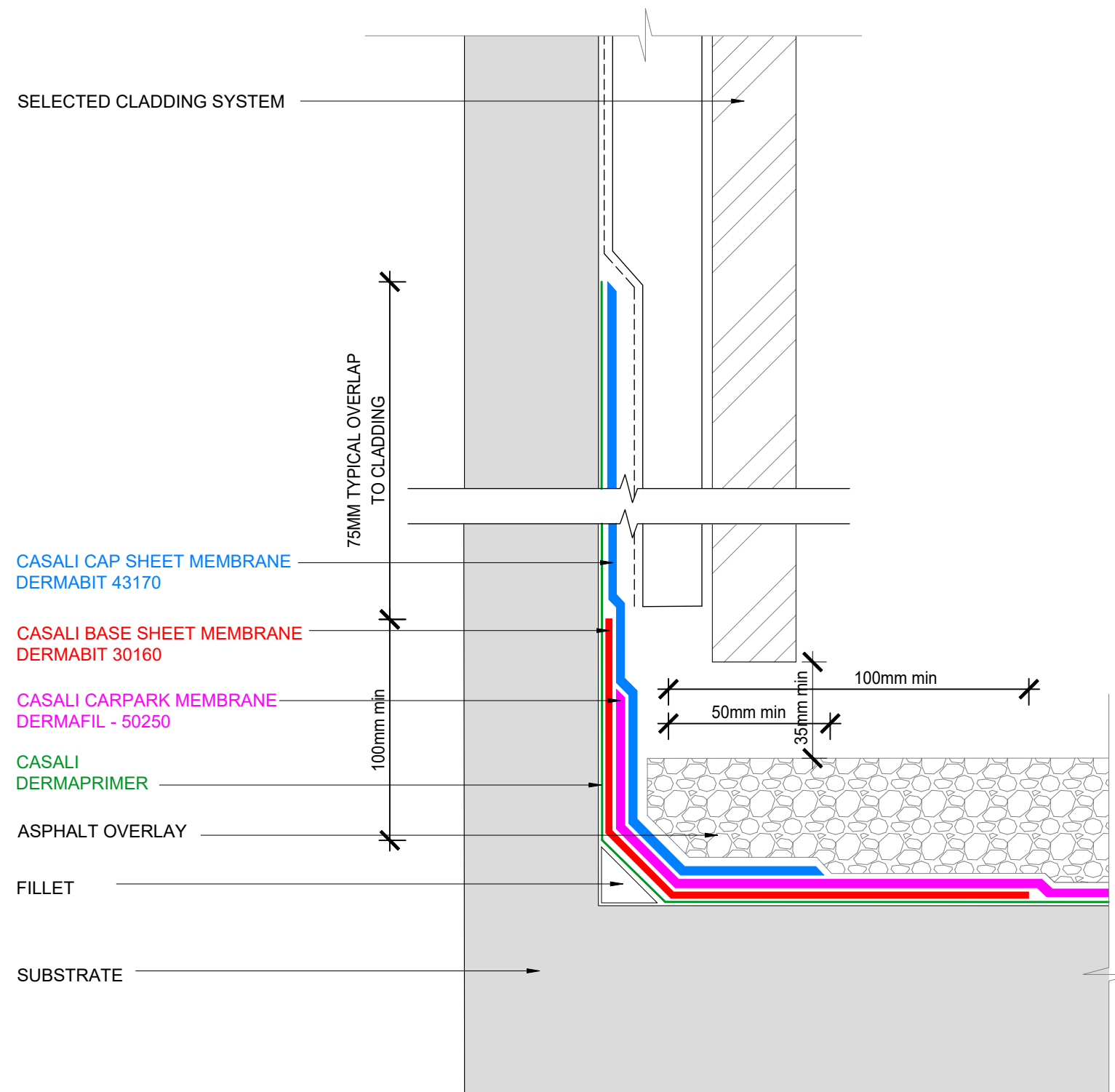
CARPARK MEMBRANE - UPSTAND BEHIND CAVITY
