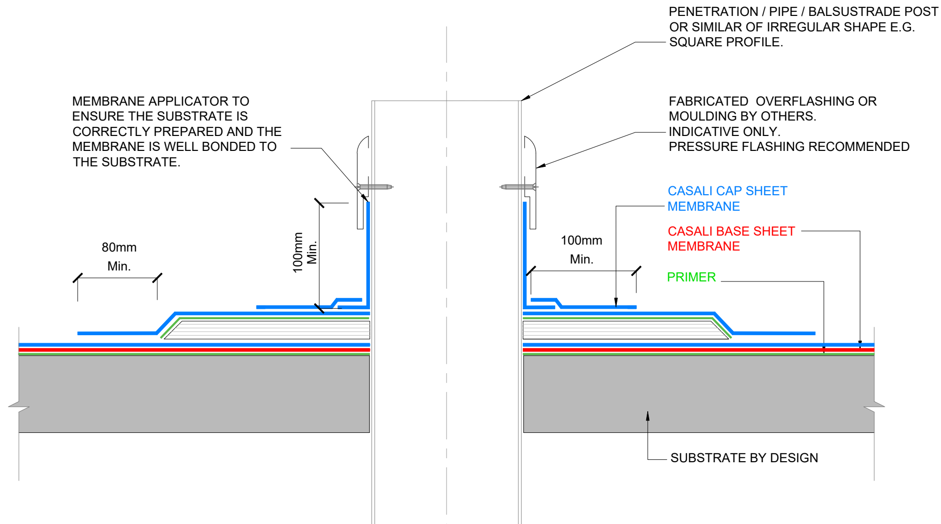
1 PENETRATION IRREGULAR SHAPES SCALE: NTS
