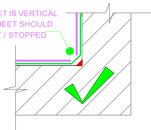
FOOTINGS / INTERNAL CORNERS
