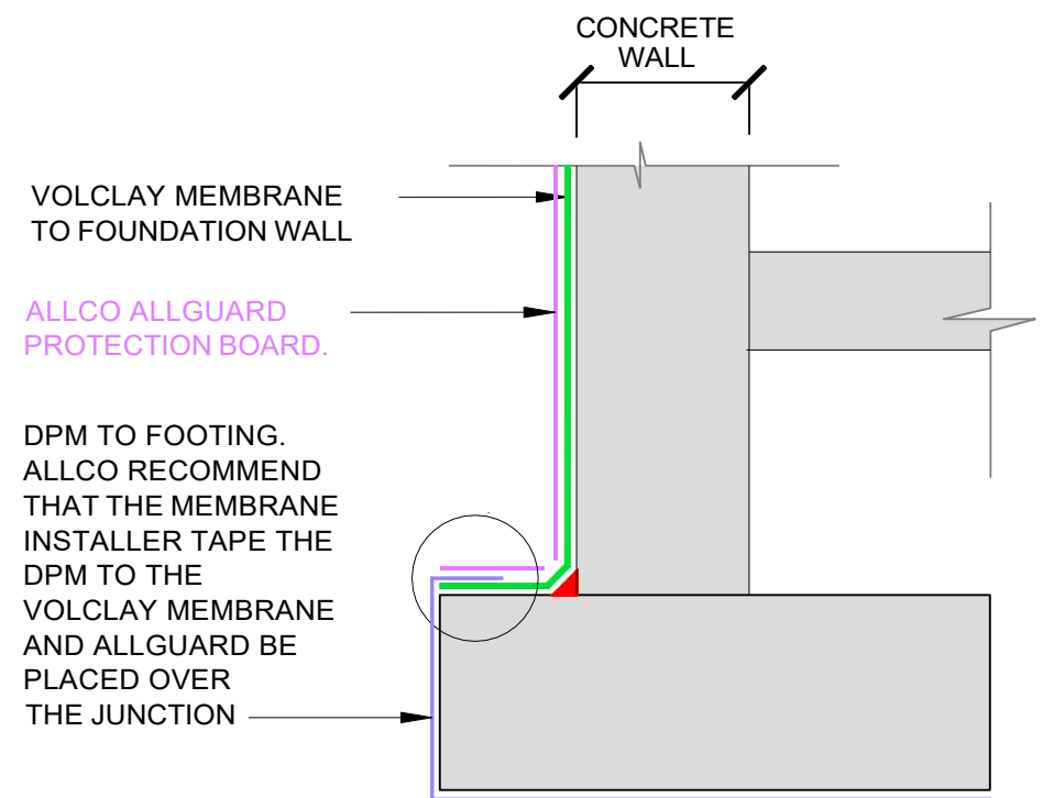
TYPICAL HEELED FOOTING EXAMPLE VOLCLAY MEMBRANE TO WALL
