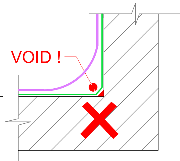
FOOTINGS / INTERNAL CORNERS
