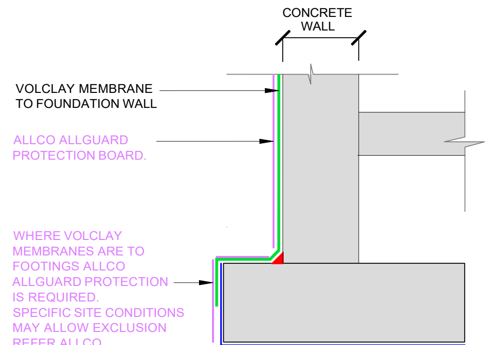
TYPICAL HEELED FOOTING EXAMPLE VOLCLAY MEMBRANE TO WALL + FOOTING
