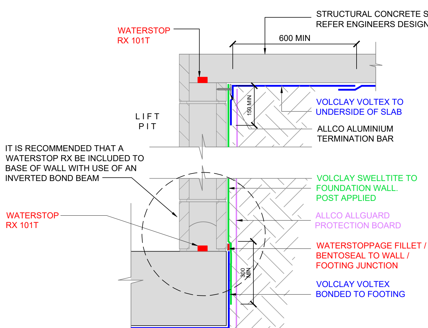
1 LIFT PIT - VOLTEX / SWELLTITE SCALE: NTS MASONRY WALLS
