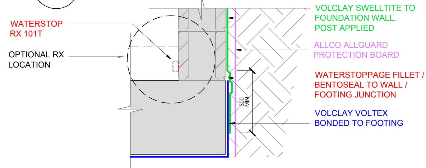
1 LIFT PIT - VOLTEX / SWELLTITE SCALE: NTS MASONRY WALLS
