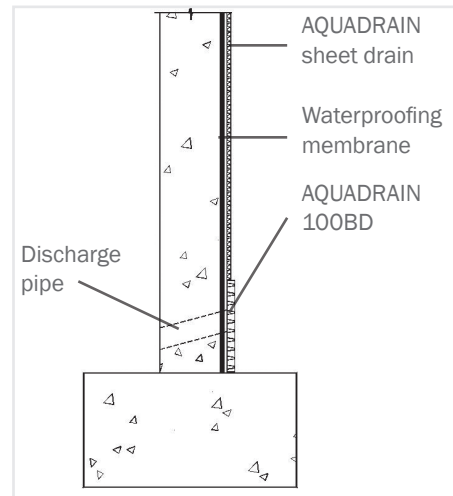
RETAINING WALL
