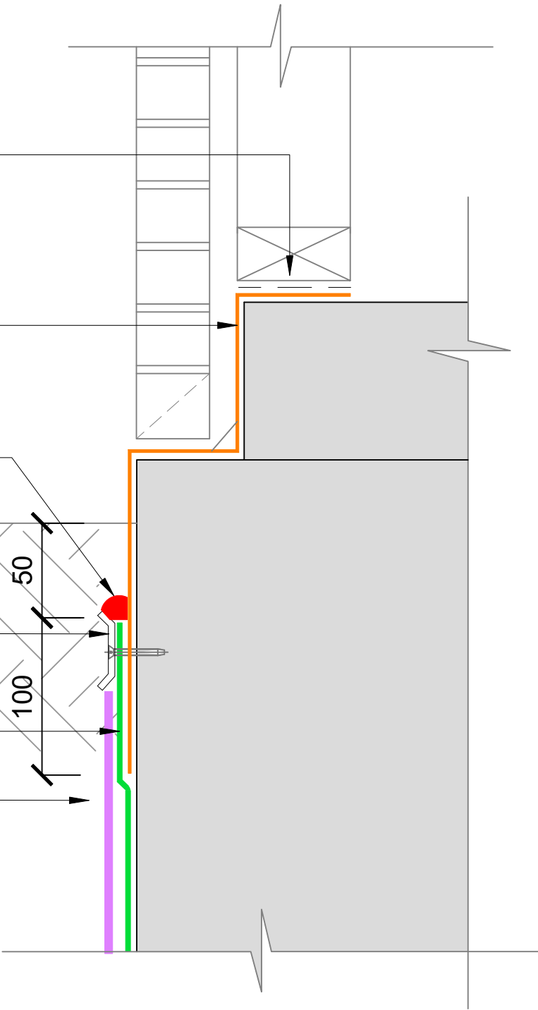
SLAB EDGE DETAIL - BRICK REBATE
