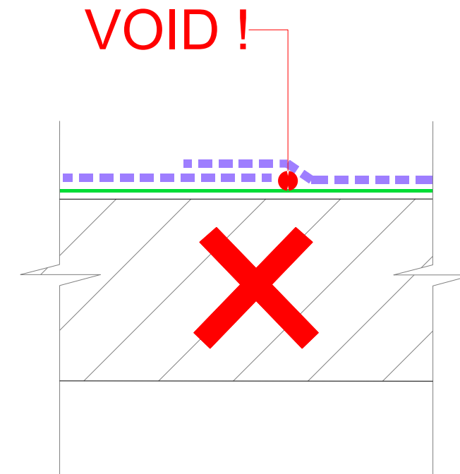
SHEET JOINTS
