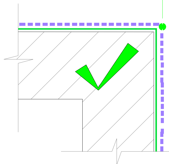
EXTERNAL CORNERS
