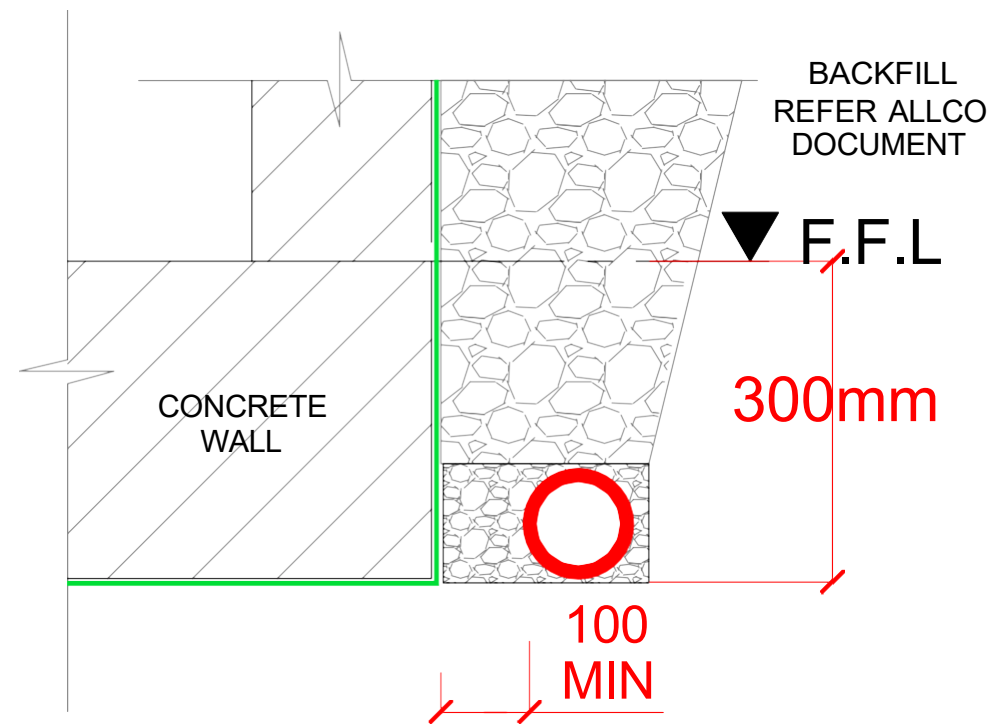
DRAINCOIL LOCATION
