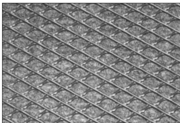
Aquadrain G20 Geonet Composite with top side filter fabric removed to show core
