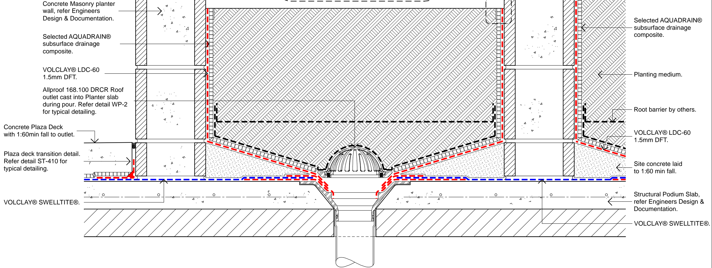
Planter Drain Scale 1:5 (A3)
