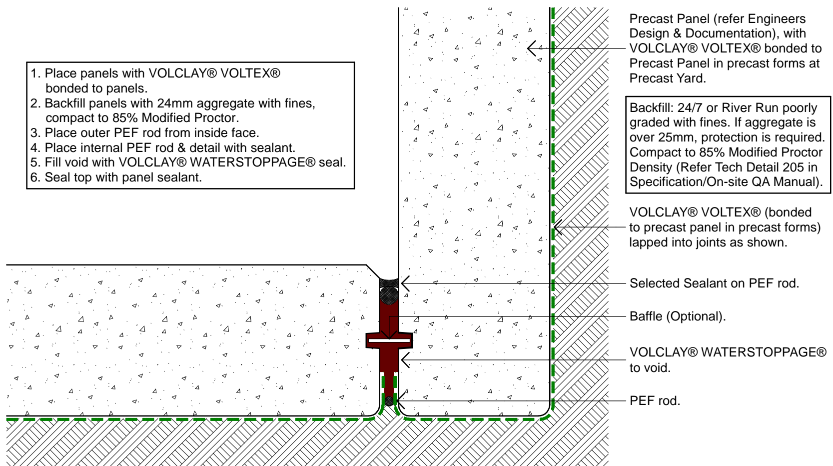
Precast Wall Corner Detail Scale 1:5 (A3)
