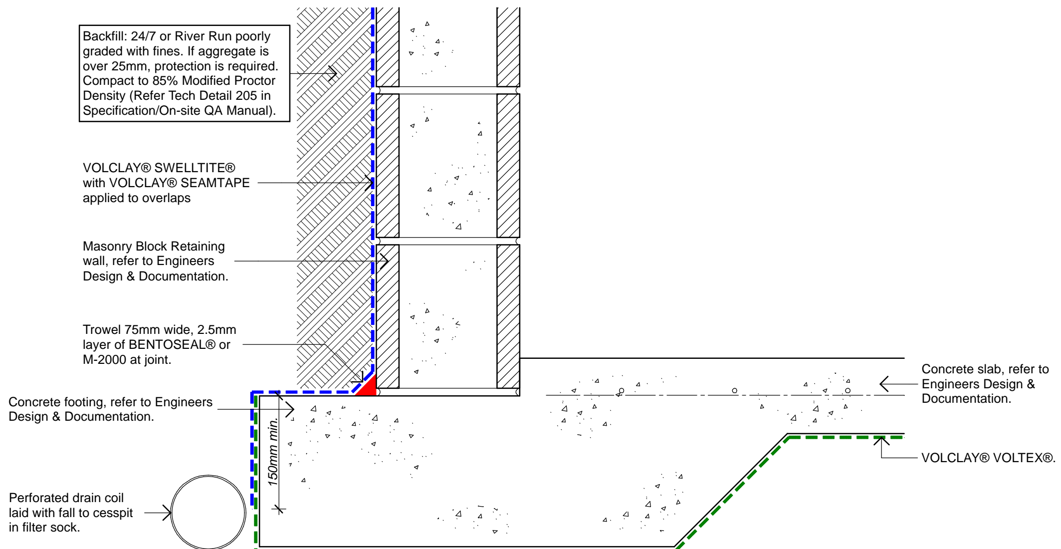
Wall With Flush Footing - Hydrostatic Scale 1:5 (A3)
