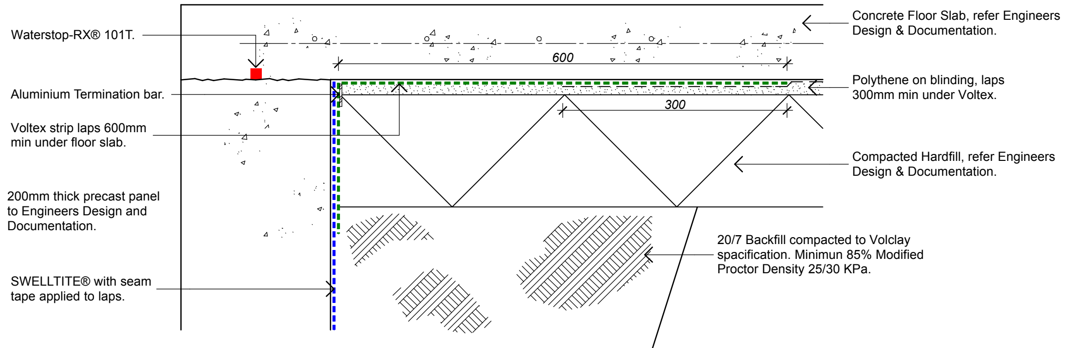
Panel To Slab Detail Scale 1:5 (A3)
